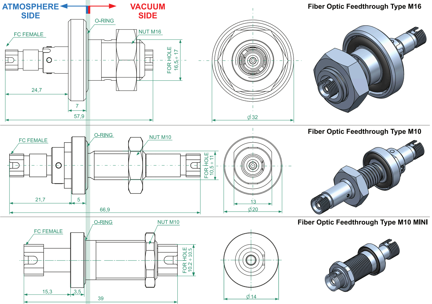
M16 Threaded Fiber Optic Feedthrough
